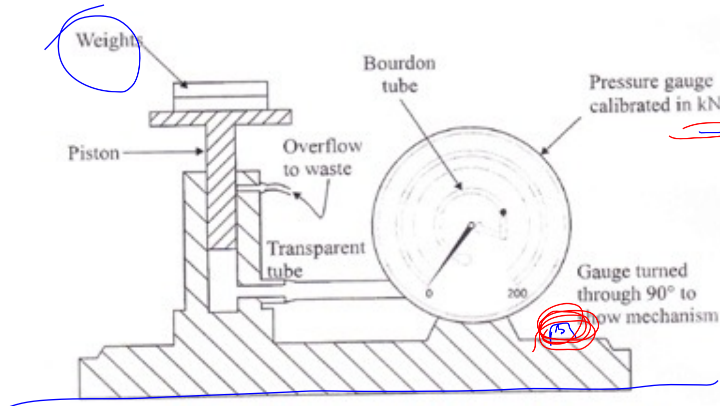
Apparatus for calibration of pressure gauge
